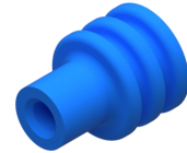
15363605 SINGLE WIRE SEAL FITS TO 8.5 mm CAVITY
